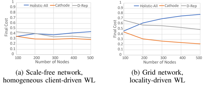
Fig. 3: Final cost after 10 epochs with static workloads as a function of system size ( N ), WL is workload.
