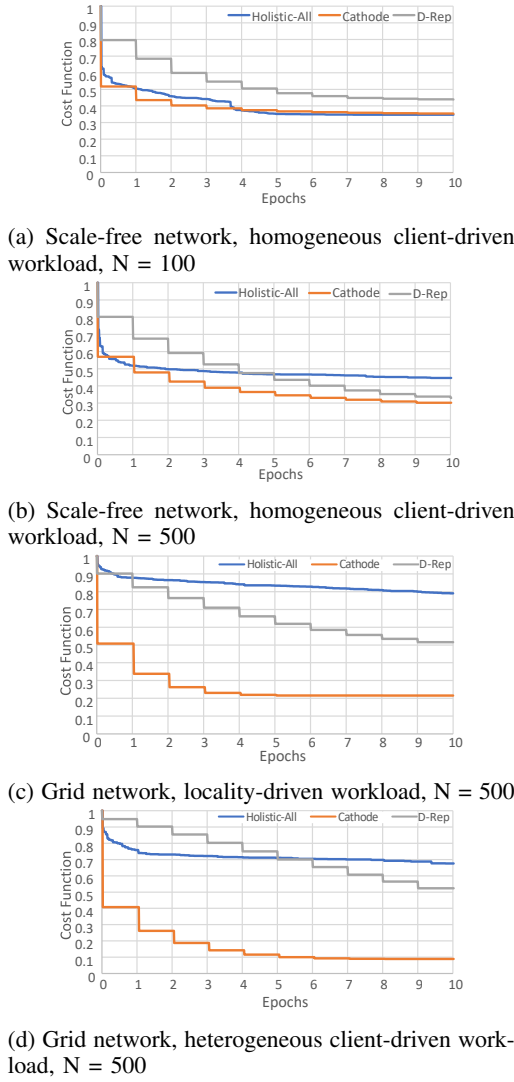
Fig. 2: Evolution of the cost function during 10 consecutive epochs with a static workload.
