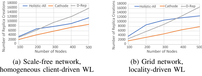
Fig. 4: Number of replica creations in 10 epochs of runtime, as a function of system size (static workloads), WL is workload.
